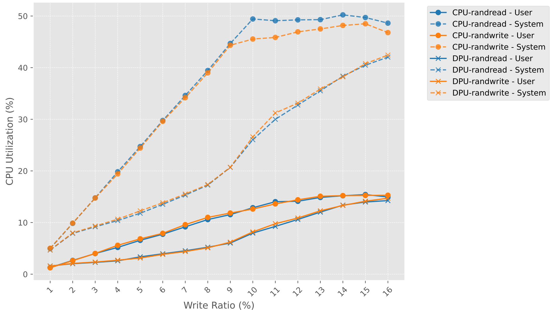
CPU Utilization vs Write Ratio (nbcpu)
